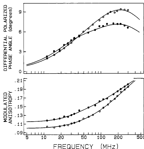
FIGURE 11: Frequency-domain anisotropy data for native and denatured TnI. Data are shown for native (●) and denatured (○, 5 M Gdn-HCl) TnI. For native TnI, \theta_1 = 0.66 ns, \theta_2 = 8.89 ns, r_1 = 0.101 , and r_2 = 0.139 . For denatured TnI, \theta_1 = 0.67 ns, \theta_2 = 7.12 ns, r_1 = 0.144 , and r_2 = 0.105 .
