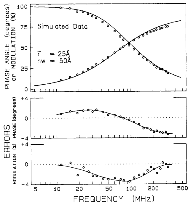
FIGURE 2: Simulated frequency response data for a D-A pair with hw = 50 \text{ Å} , R_0 = 20 \text{ Å} , \bar{r} = 25 \text{ Å} , and \tau_D = 3 \text{ ns} . The solid lines show the best single exponential fit and the lower panels the deviations from this model, \chi_R^2 = 52.7 .
